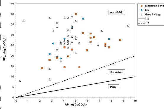
Figure 13: Acid rock drainage (ARD) potential is assessed using neutralization potential ratios
