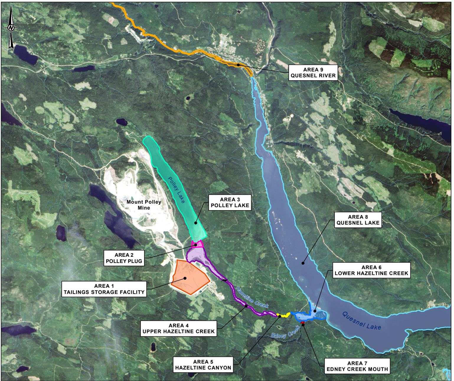
Figure 3: Remediation areas: Mount Polley Mine TSF dam failure
