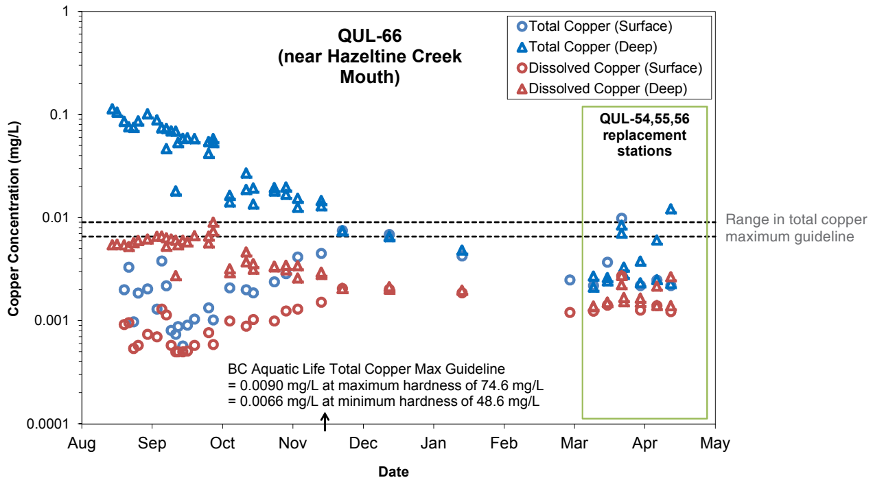
Figure 16: Post-event measurements of total and dissolved copper in Quesnel Lake near Hazelline Creek
